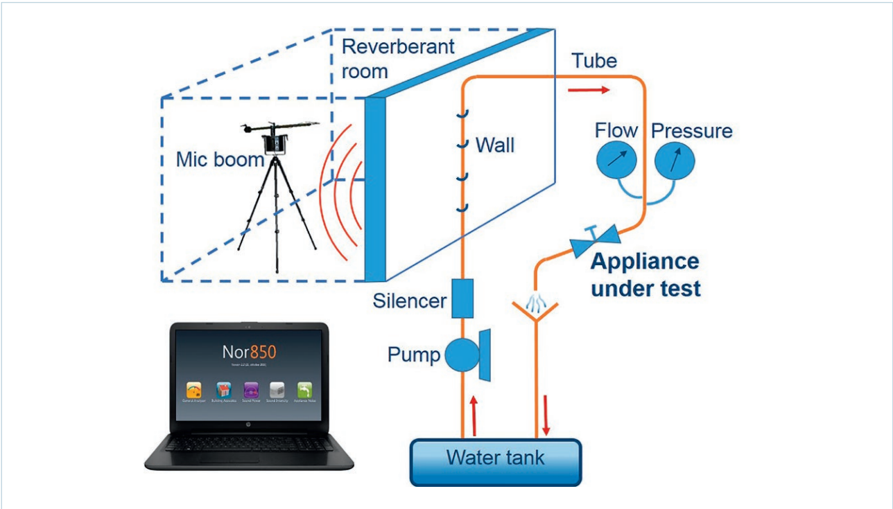
ISO 3822 setup
